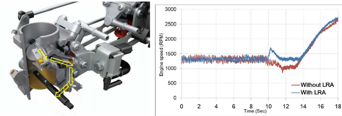
Engine rpm in launching moment
