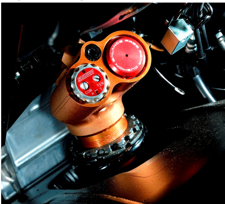
BFRC lite shock absorber damping adjustment controls.
