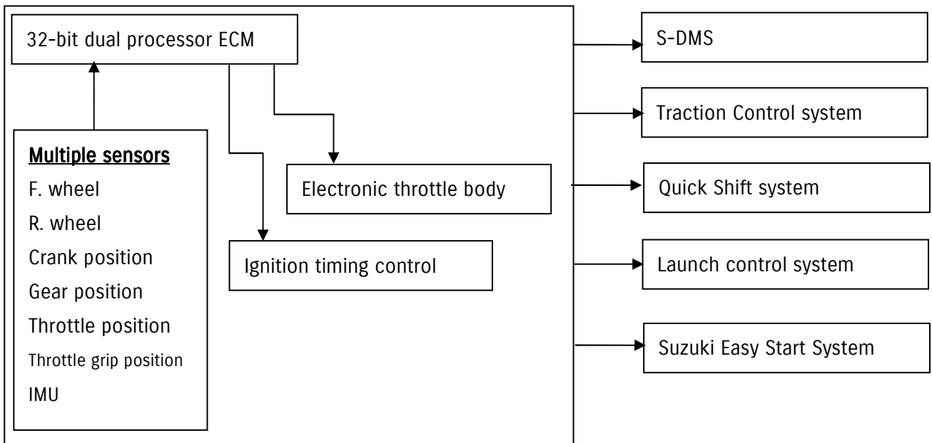
32-bit dual processor ECM
