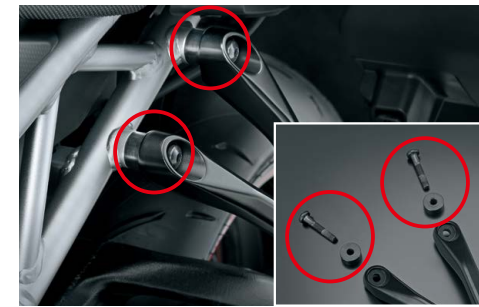
Side Case Adapter 93900-48810-000 Required for installing Side Case (Left).
